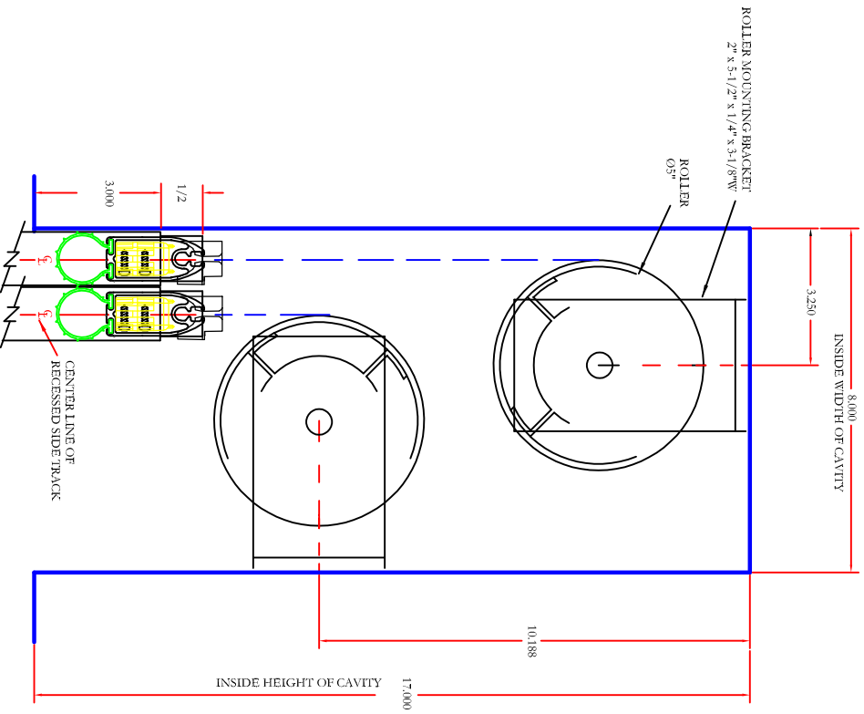
PLACEMENT OF 2 - 5" ROLLERS IN A CAVITY STACKED ONE ABOVE THE OTHER WITH RECESSED SIDE TRACK
